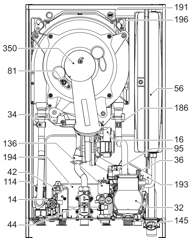
fig. 40- Vista general
