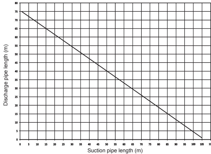
MAXIMUM STRAIGHT LENGTH Ø 80
